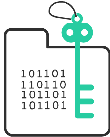
ICSF View
