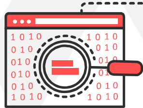
DFSMS View
