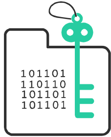
ICSF View
