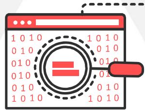
DFSMS View
